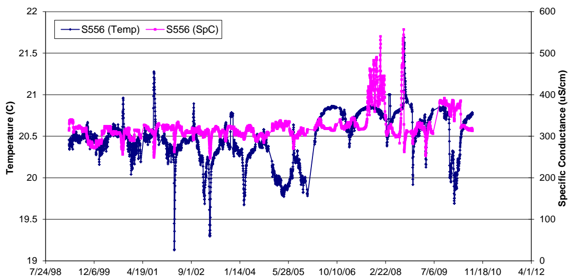
Figure 4-1. Wakulla Spring average daily temperature and specific conductance time series (source NFWFMD).
